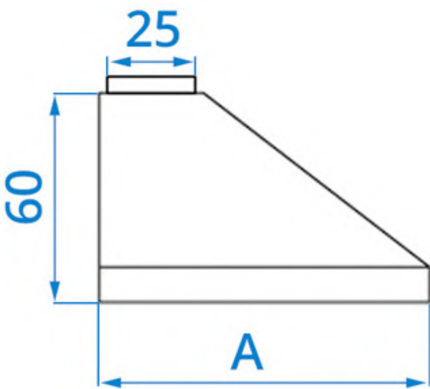
VISTA FRONTAL
