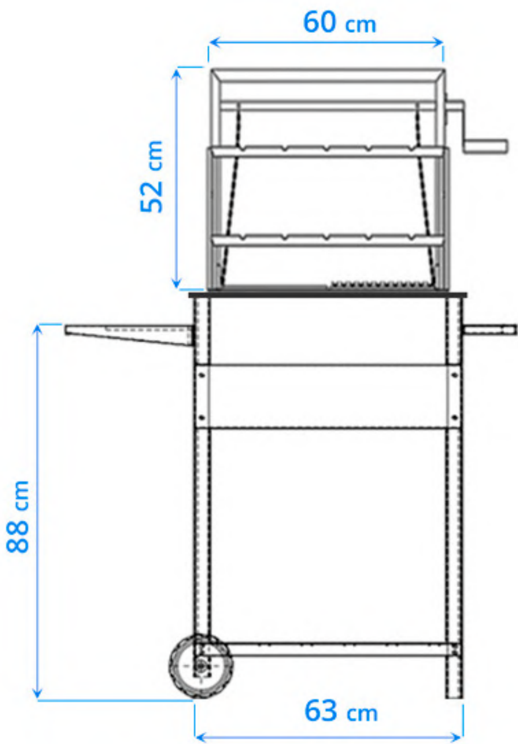
VISTA FRONTAL
