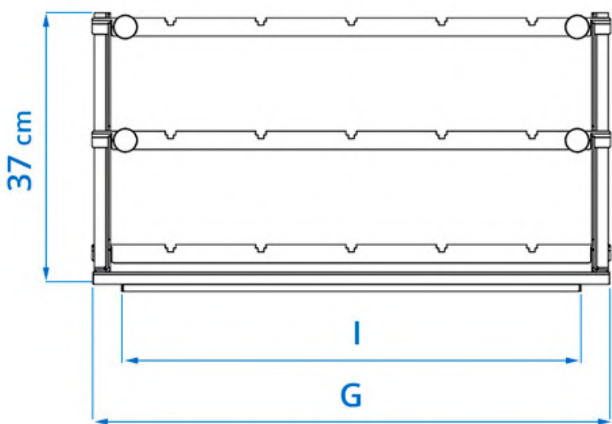
VISTA FRONTAL
