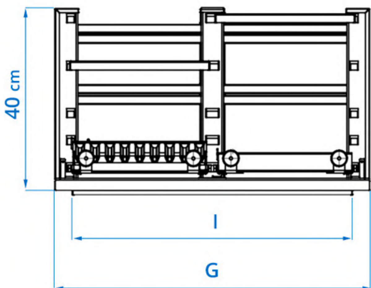
VISTA FRONTAL
