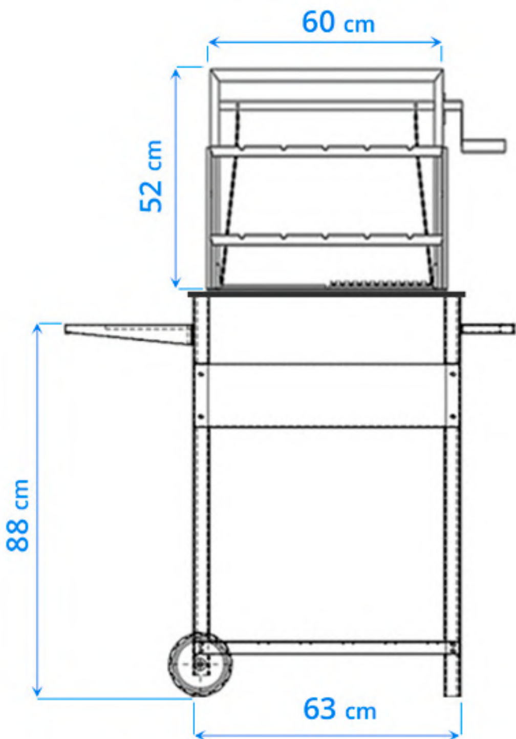
VISTA FRONTAL
