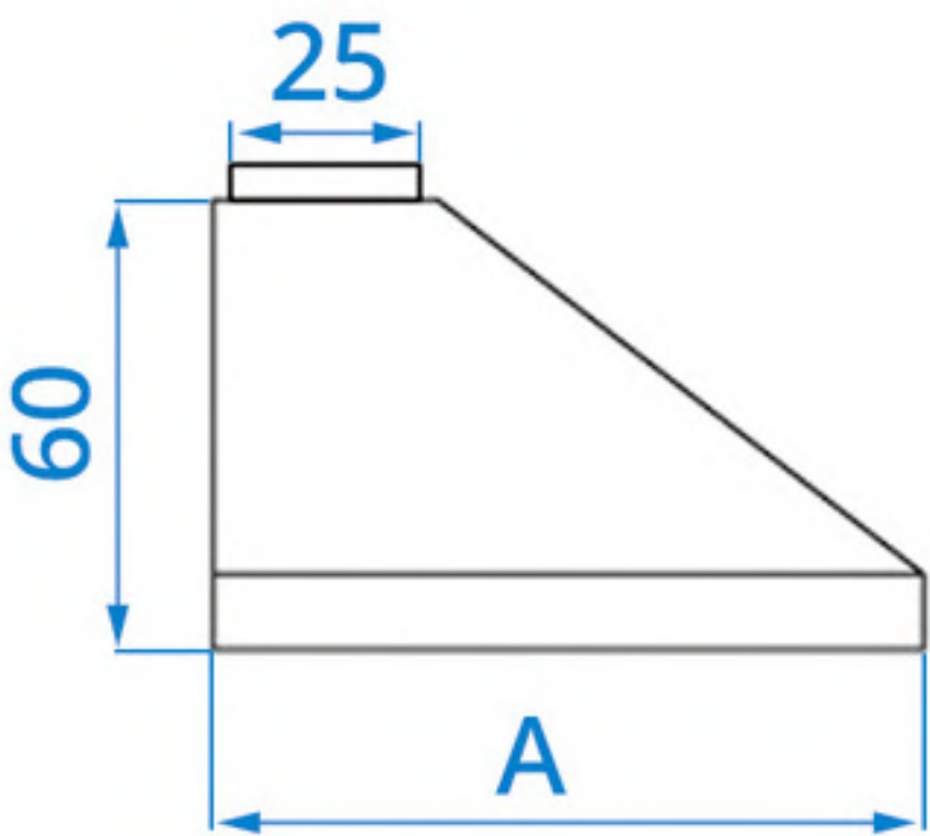
VISTA FRONTAL
